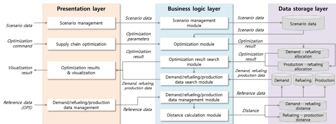
Fig. 4 – System architecture.
